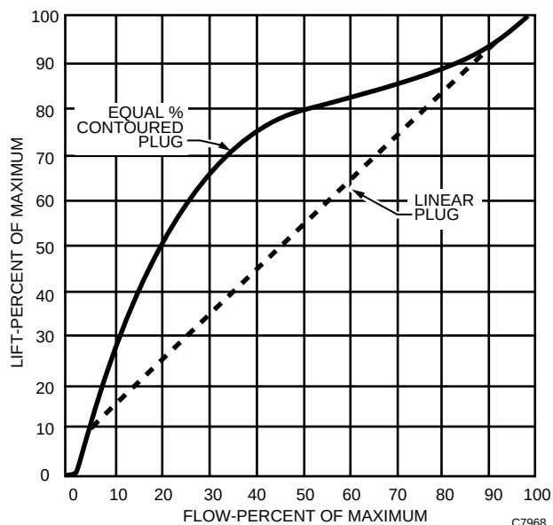
Fig. 1. Typical Flow Characteristics.
