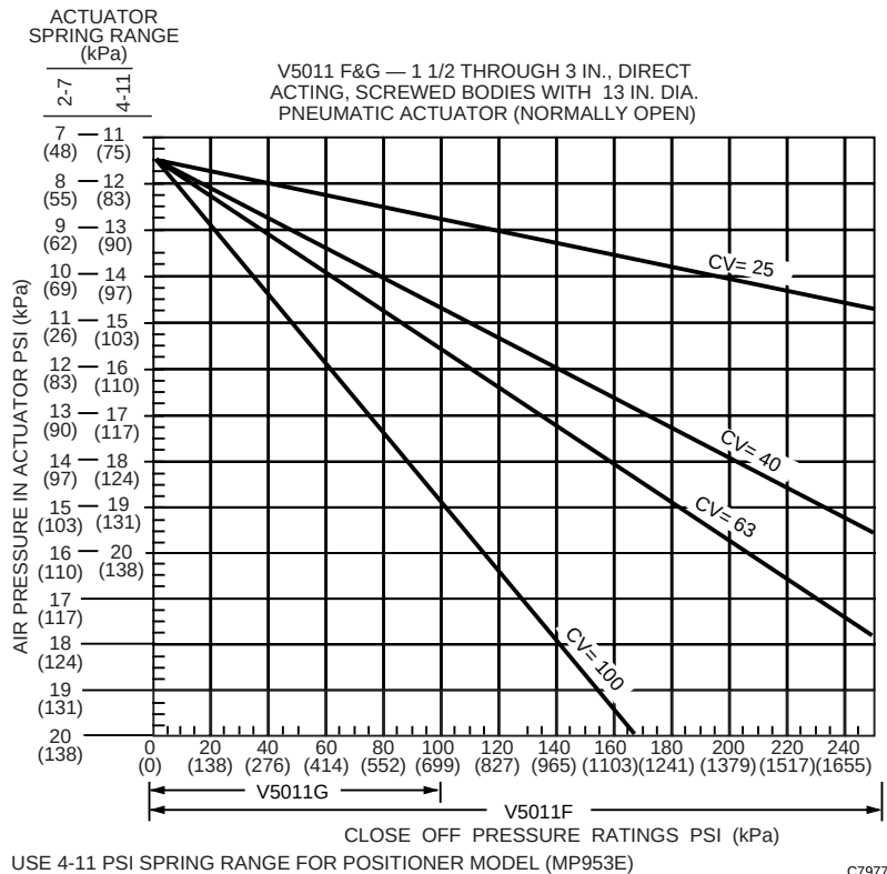
Fig. 7. Close-Off Pressures at Various Control Air Pressures for V5011 Valves and MP953 Pneumatic Actuators. (Continued)
